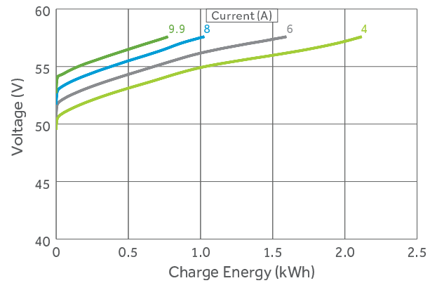
Voltage vs. Charge Energy
